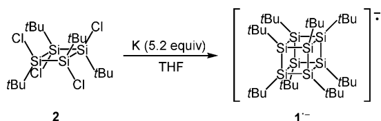
Scheme 2. Generation of 1 •− by the reduction of 2 .
